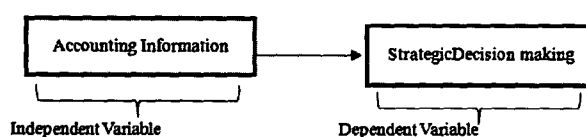
Fig 1: theoretical framework
