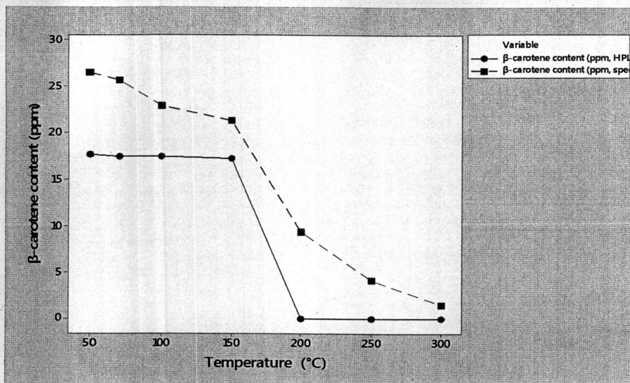
Figure 3 Stability of β-carotene at higher temperatures in M. longifolia seed oil.
