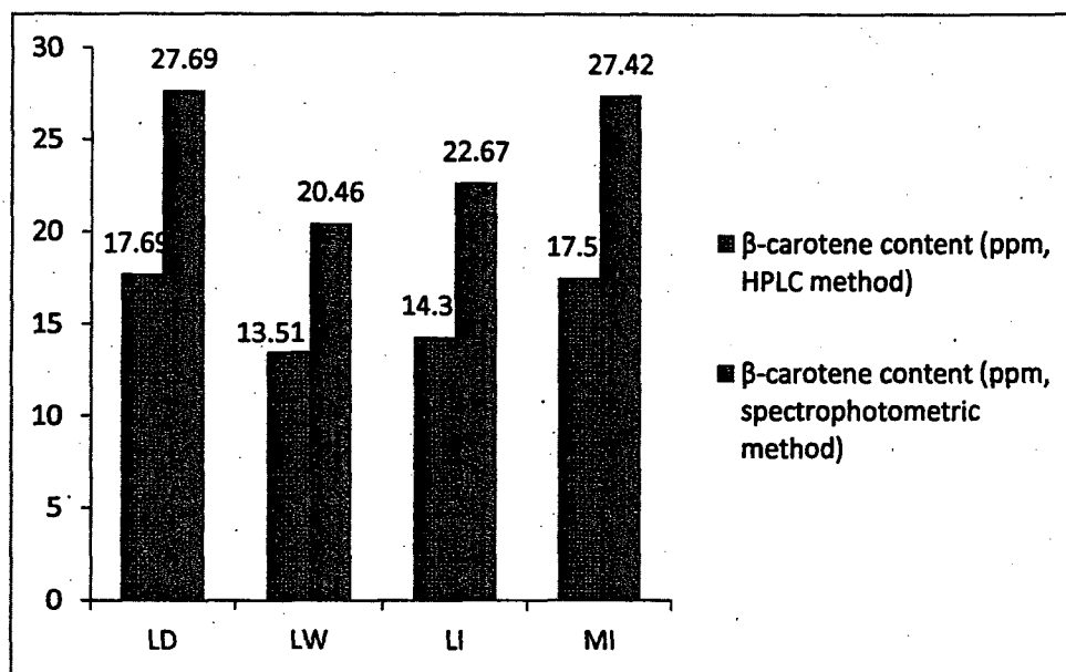
Figure 1 β-carotene content (ppm) of M. longifolia seed oil in four agro-climatic zones.
