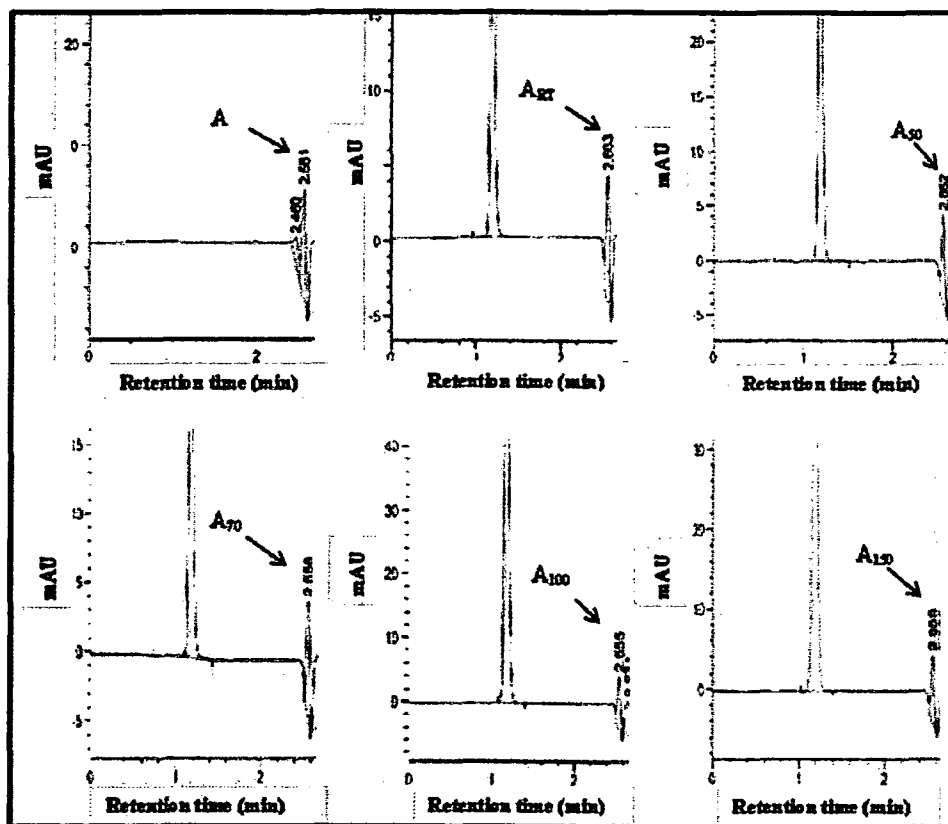
Figure 2 Peaks for \beta -carotene in HPLC chromatogram for standard (A), at room Temperature ( A_{RT} ), at 50 °C ( A_{50} ), at 70 °C ( A_{70} ), at 100 °C ( A_{100} ) and at 150 °C ( A_{150} ).
