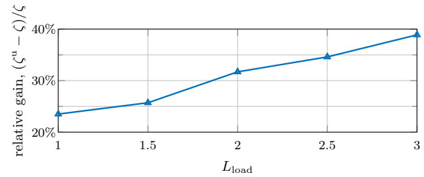
Figure 10. The relative gain of the proposed heuristic compared with the benchmark in the German network as the traffic load L_{load} changes.
