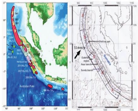
Figure 1: The map showing the study region. Left: Rupture areas of large earthquakes took place in the Sumatra subduction zone. Closed areas show the re-ruptured regions and dashed areas show the seismicity gaps. Right: Outer-rise, near trench and shallow part in the study region and sub-regions A, B, C, D and E.
