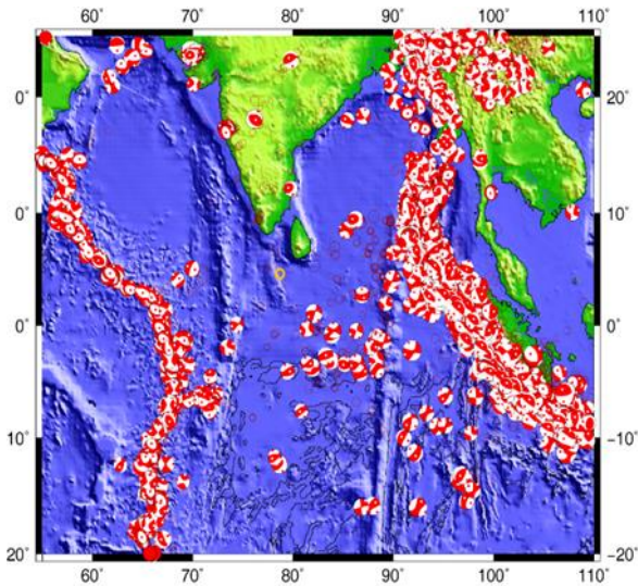
Figure 2: Focal mechanism solutions data in the offshore Sri Lanka obtained from the Global Centroid Moment Tensor database, catalog for the earthquakes of magnitude greater than 3.5 occurring from 1976 to 2011.
