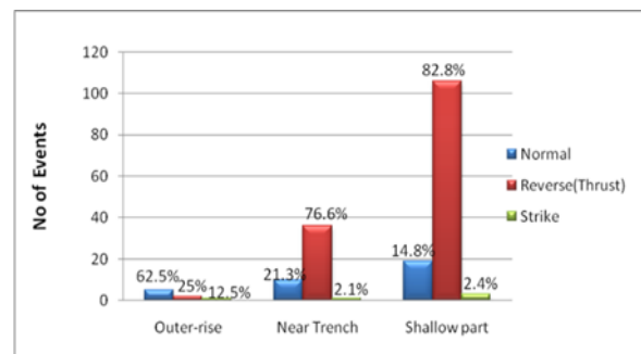
Figure 3: Distribution of number of events in faults with respect to the regions, outer-rise, near
